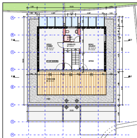
GRUNDRISS ATTIKAGESCHOSS
